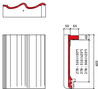
chaperonpan 90°
