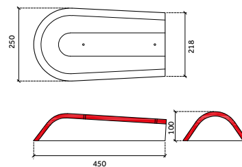
euro-hoekkeperbeginvorst
