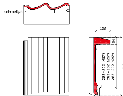
chaperonpan 90°
