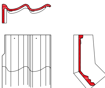
knikgevelpan links 140°
