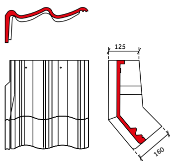
knikgevelpan links 140°
