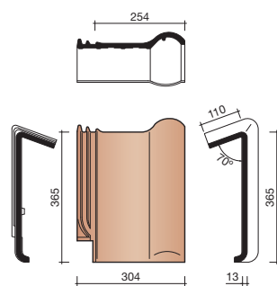
8500 CHAPERONPAN
