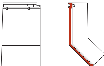
knikgevelpan 140° links
