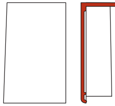
chaperongevelpan links 90°
