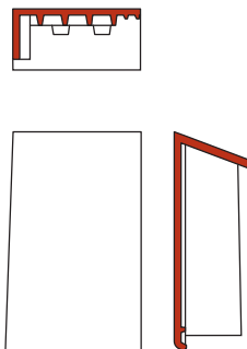
chaperongevelpan 70° links
