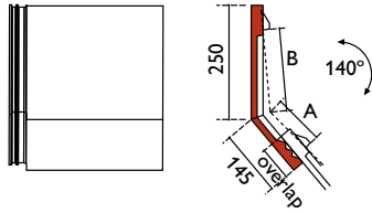
knikpan 140°
