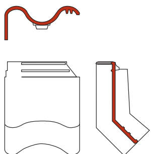
knikgevelpan links
