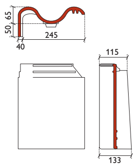
gevelpan links
